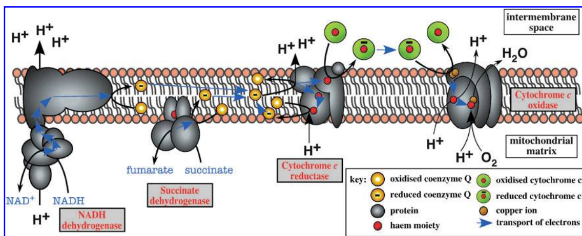
FIG. 2. The mitochondrial ETC that occurs in the inner mitochondrion membrane of most eukaryotes. The inner membrane contains several dehydrogenases, including NADH dehydrogenase (complex I) and succinate dehydrogenase (complex II), which feed electrons from various sources to coenzyme Q (yellow), a molecule embedded within the membrane. Reduced coenzyme Q donates electrons to cytochrome c reductase (complex III). These electrons pass through several metal-based reaction centers, including heme (red), and ultimately reduce the heme prosthetic group of cytochrome c (green). Cytochrome c is a motile intermembrane space protein that donates electrons to cytochrome c oxidase (complex IV). Cytochrome c oxidase contains several metal centers, including two copper ions (orange) and two heme moieties, which ultimately donate electrons to oxygen, the terminal electron acceptor in the chain. The ETC generates a proton gradient and membrane potential across the inner membrane, which has several critical functions in the mitochondrion, including in the generation of ATP via an F-type ATP synthase. ATP, adenosine triphosphate; ETC, electron transport chain; NADH, nicotinamide adenine dinucleotide.
